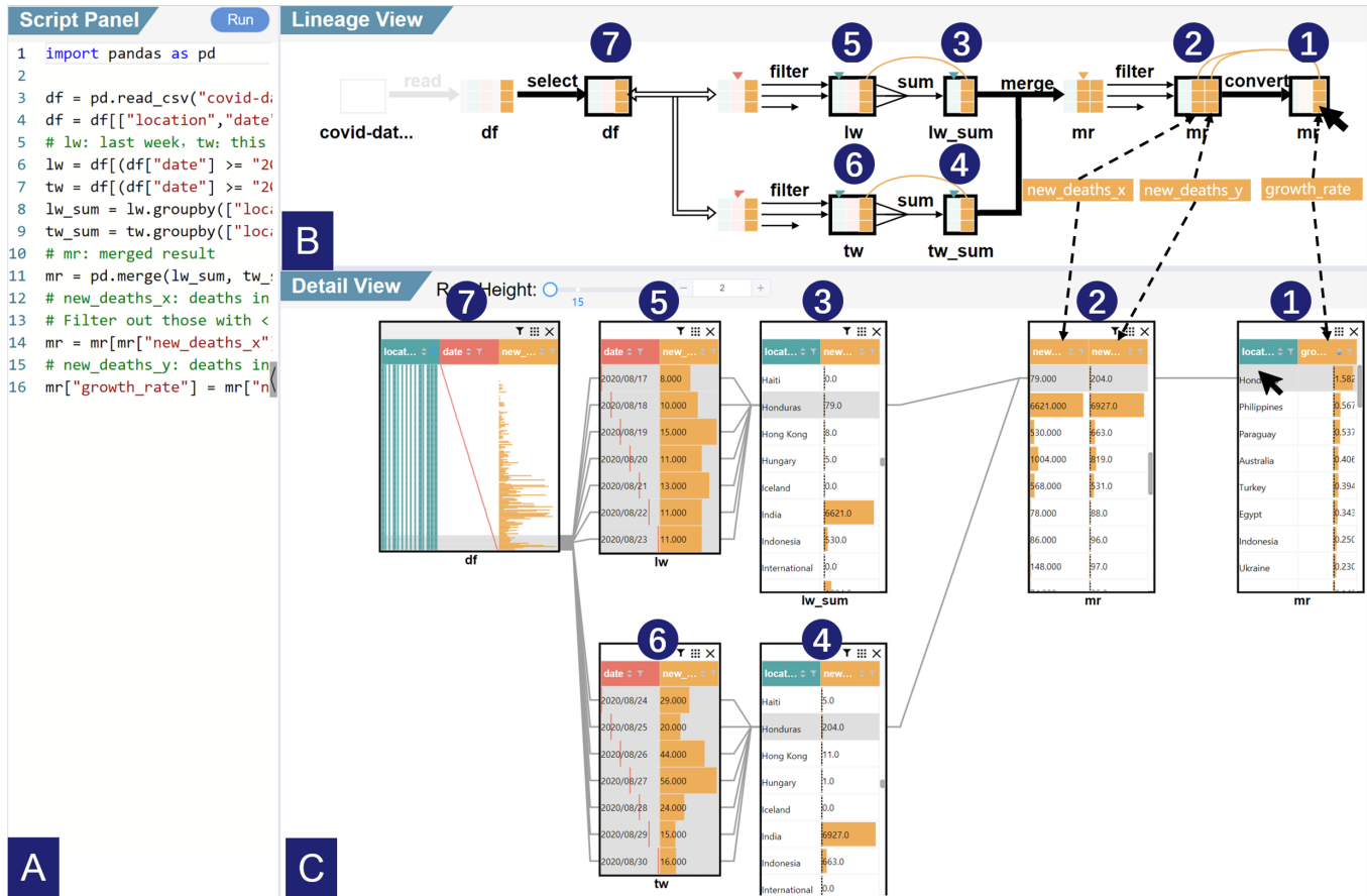
Fig. 7. HYPNOS presents the DL extracted from a data transformation script for analyzing the trend of Coronavirus deaths at different levels of detail. The interface consists of (A) a script panel which shows the script, and two visualization components: (B) a lineage view for presenting the data pipeline, which supports table-level and column-level DLT; (C) a detail view for presenting the intermediate tables in the data pipeline, which supports row-level DLT and allows users to inspect details.
