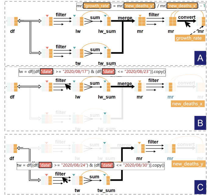
Fig. 8. Column tracing of growth_rate (A), new_deaths_x (B), and new_deaths_y (C). Hovering on the edges, users can see the code while highlighting the critical columns.
