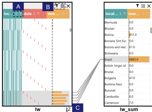
Fig. 5. Visual encoding for different data types in the detail view and the result of tracing data items.
