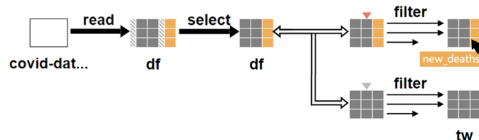
Fig. 4. Applying glyphs to the lineage graph. This figure shows the focus mode for coloring.
