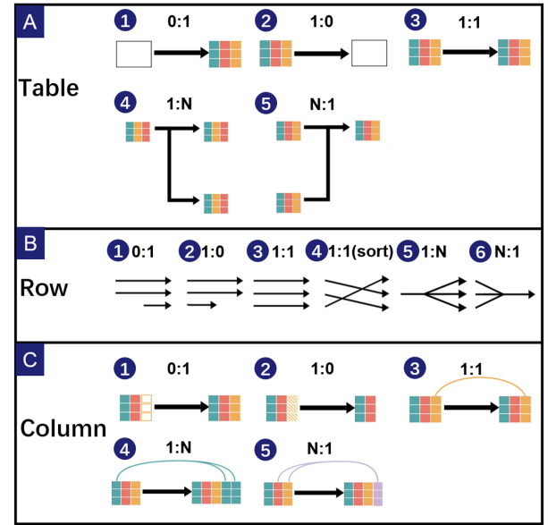
Fig. 2. Visual representations of different types of data transformations. We use rectangles and arrows to represent table-wise (A) and row-wise (B) data changes and relationships. We use curves to indicate column-wise value changes (C).
