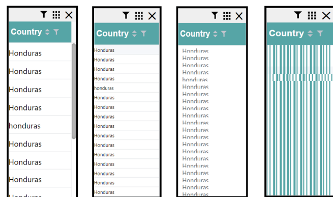
Fig. 6. The Comparison of various approaches for showing categorical data. (A) a larger font size results in less items displayed; (B) a smaller font size results in poorer readability; (C) a normal font size with less row height results in occlusion; (D) barcodes show grouped identical items.
