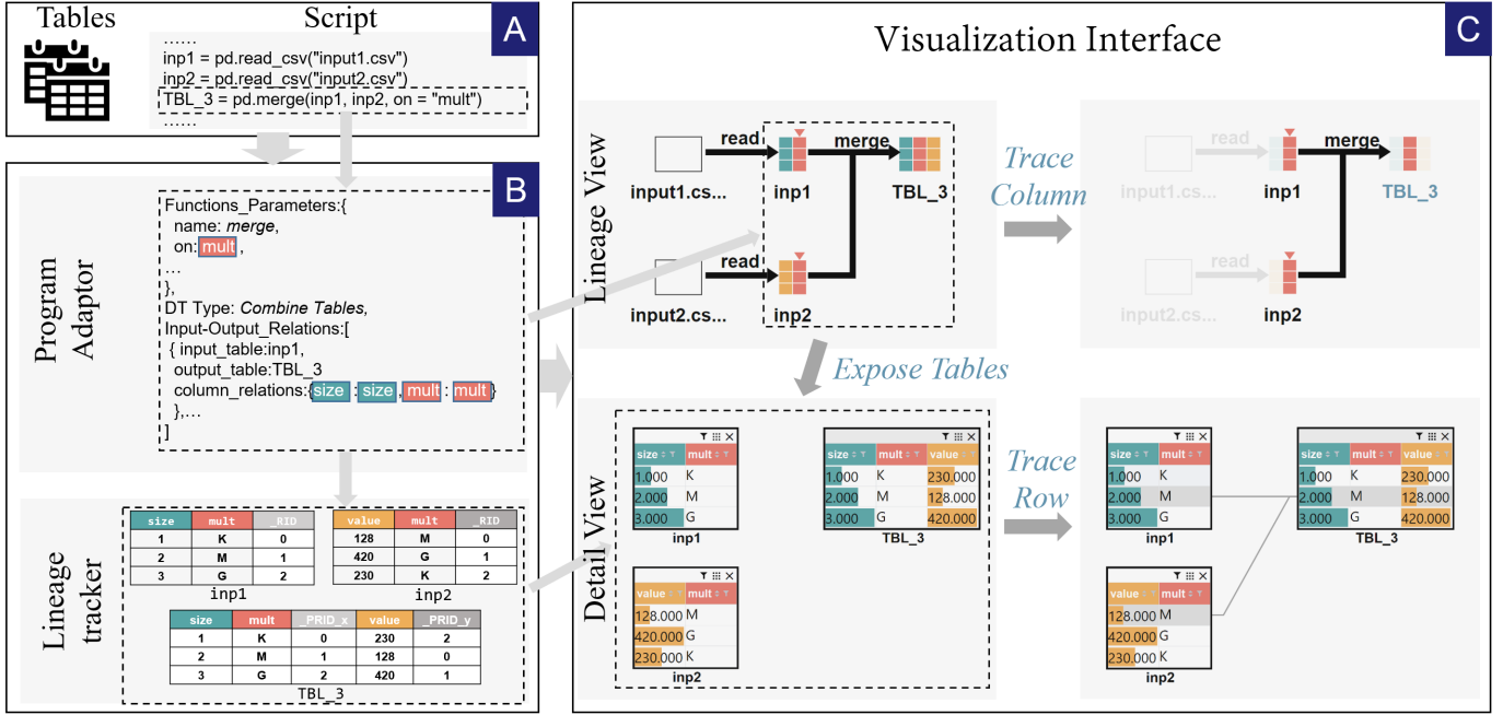
Fig. 1. The architecture of HYPNOS. HYPNOS takes a DT script and the underlining table files as input (A). The lineage module (B) consists of a program adaptor for adapting code and a lineage tracker for capturing DL. The visualization interface (C) consists of a lineage view and a detail view for supporting schema-level and instance-level DLT tasks, respectively.
